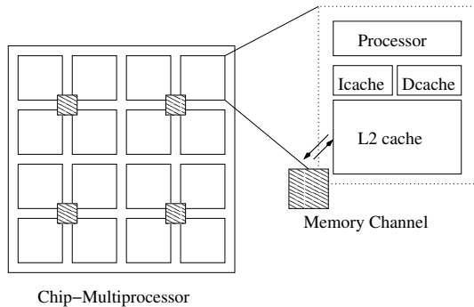
Figure 1. Chip-multiprocessor model.
