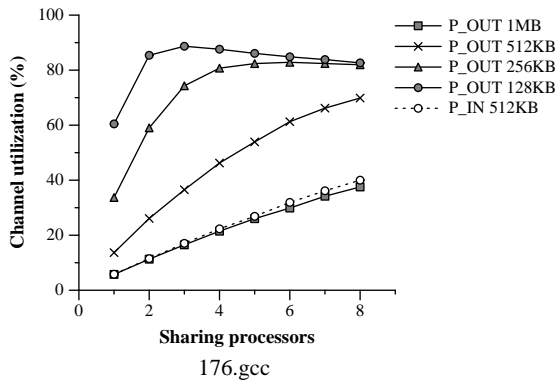
Figure 6. Channel utilization (%) versus channel sharing.
