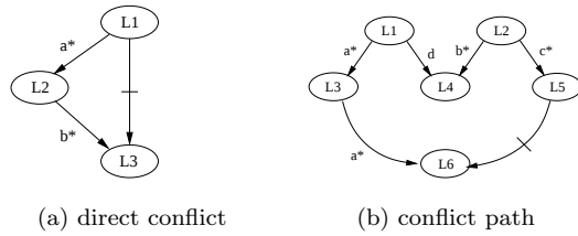
Figure 3. Conflict Between Potentially Removable Arrays
