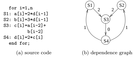
Figure 4. Modeling dependences in a loop
