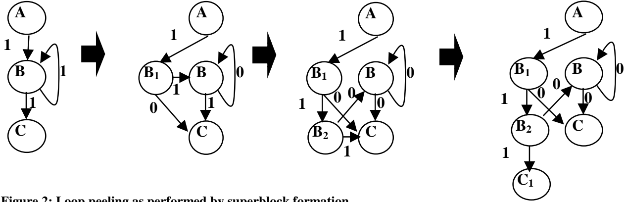
Figure 2: Loop peeling as performed by superblock formation
