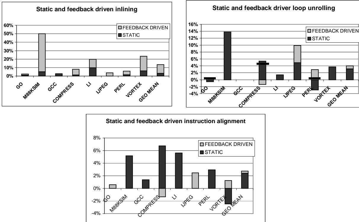
Figure 6: Static and feedback driven optimizations
