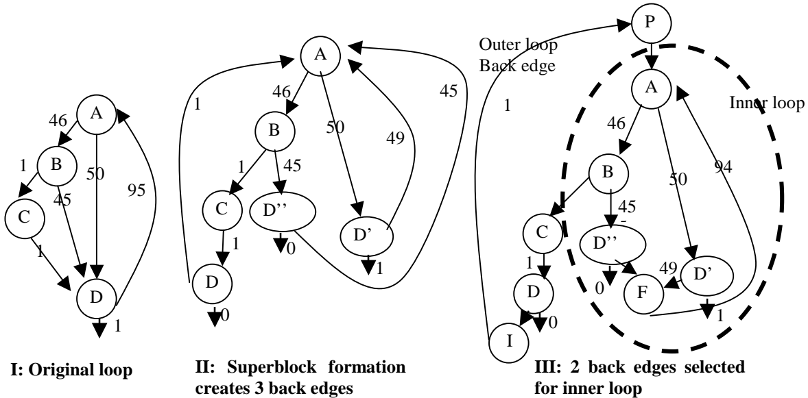
Figure 1: Superblock formation followed by commando loop optimization. Flow-graph edges are annotated with execution counts
