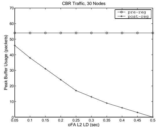
Figure 13 Peak buffer usage varying L2 LD
