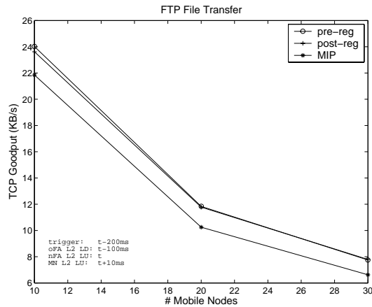
Figure 14 TCP Goodput
