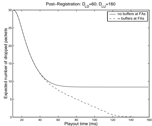
Figure 5: Post-Registration
