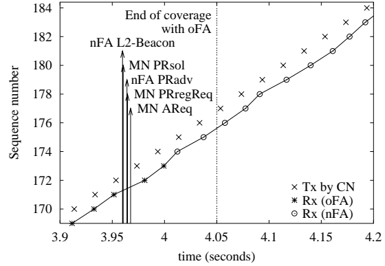
Figure 3: Target Trigger-Pre Registration handoff.
