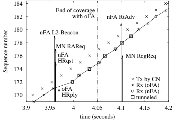
Figure 2: Target Trigger-Post Registration handoff.
