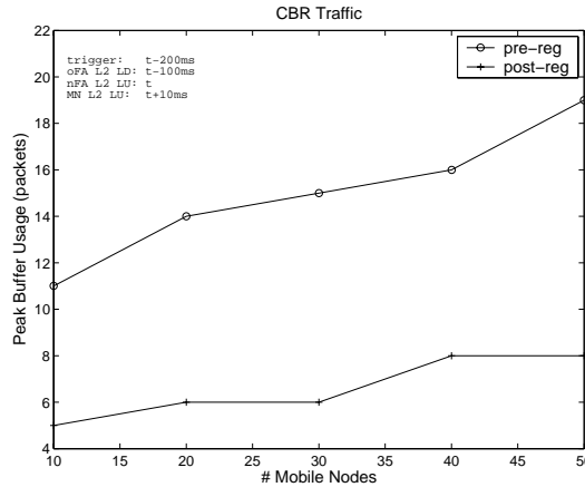
Figure 11 Peak buffer usage
