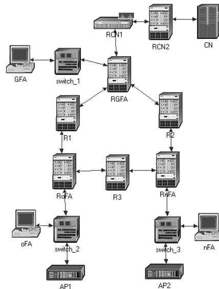
Figure 10 OPNET Network Model
