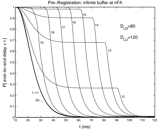
Figure 6: Individual delays – Pre
