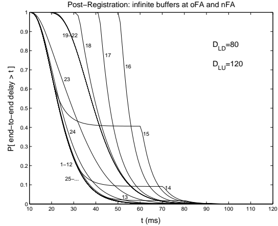
Figure 7: Individual delays – Post
