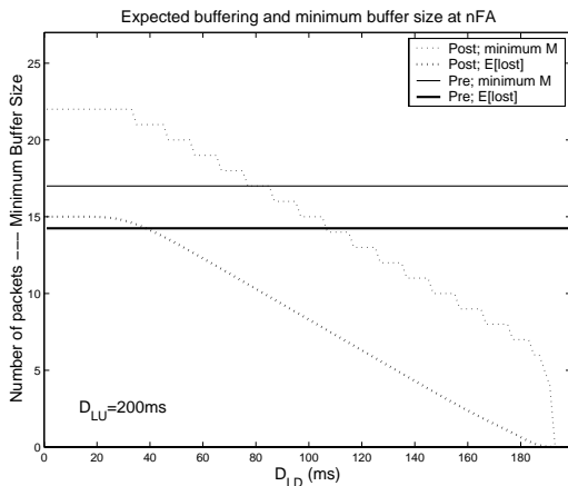
Figure 8: Buffering in nFA
