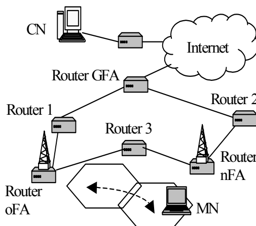
Figure 1: Reference Network
